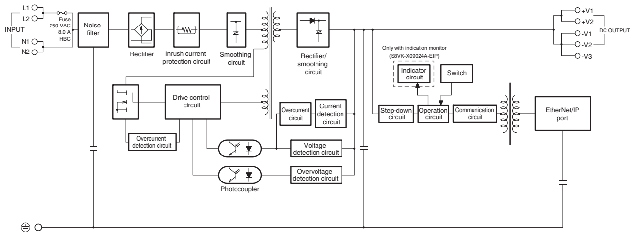
S8VK-X12024-EIP
